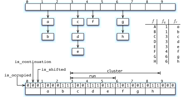
Figure 1: An example quotient filter and its representation. This filter contains values A through H. The table on the right shows, for each value, the corresponding quotient and remainder. The top of the figure shows a chained hash table storing the values A through H by storing a list of remainders in a bucket identified by the quotient of the values. The bottom of the figure shows how the remainders are stored in the QF. Each bucket contains three bits in addition to the remainder. The three bits are the is_occupied , is_continuation , and is_shifted values, in that order. In this example, C, D, and E have all the same quotient, so together they form a run. Value C is stored in its canonical position, so it is the beginning of a cluster. Although F should have been stored in bucket 4, it is pushed forward by D and E to bucket 6. Values C through H together form a cluster.
